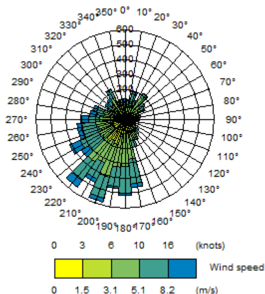
Figure E3.3 Wind rose for Teesside International Airport, 2019
